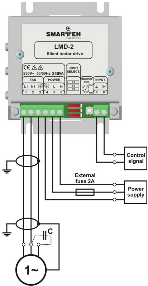
Figure 2: Connection scheme
