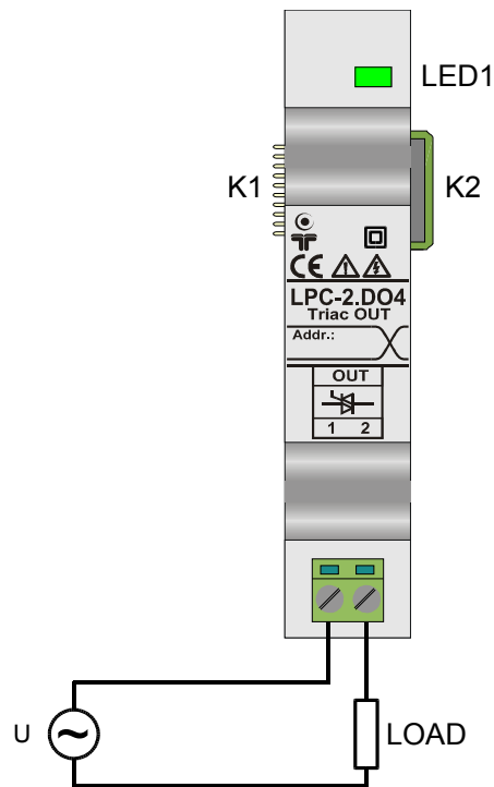
Figure 2: Connection scheme
