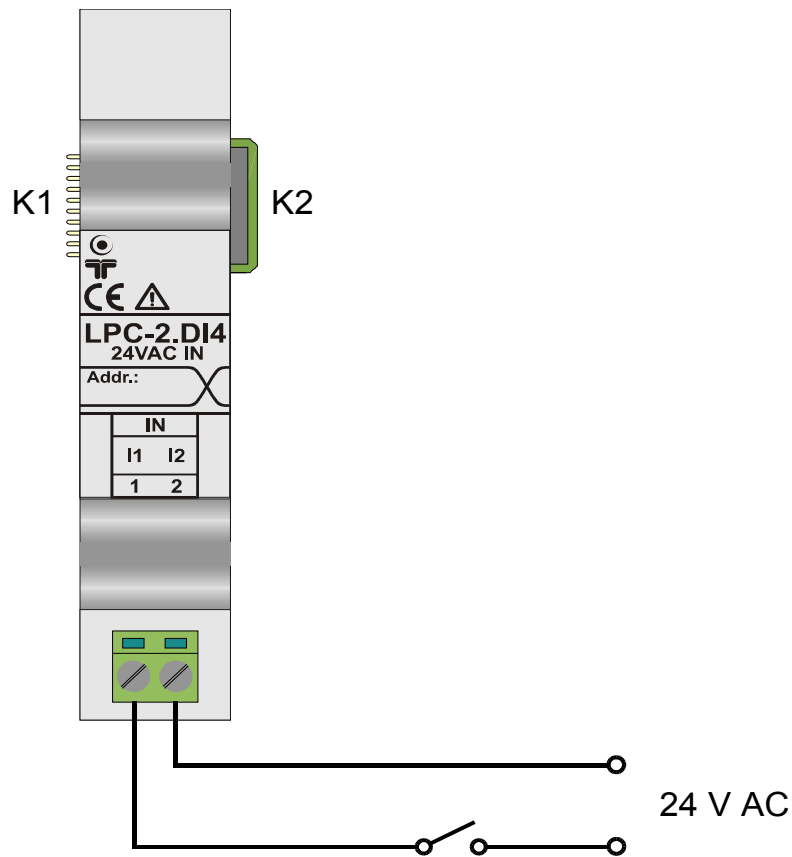
Figure 2: Connection scheme
